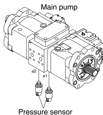
Pressure sensor
